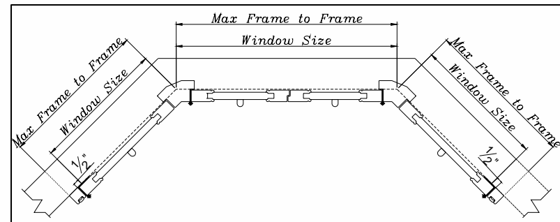
Hang Strip Outside Mount
